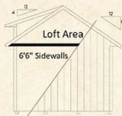
6'6" Sidewalls - 8 Pitch - Loft
