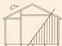
Standard 6'6" Sidewalls - 4 Pitch - No Loft
